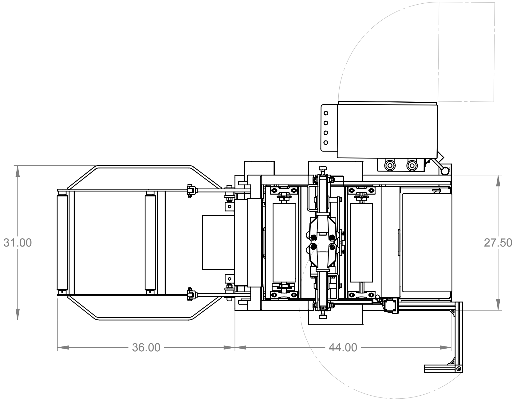
NDT III FOOTPRINT TIRE LIFT DOWN
